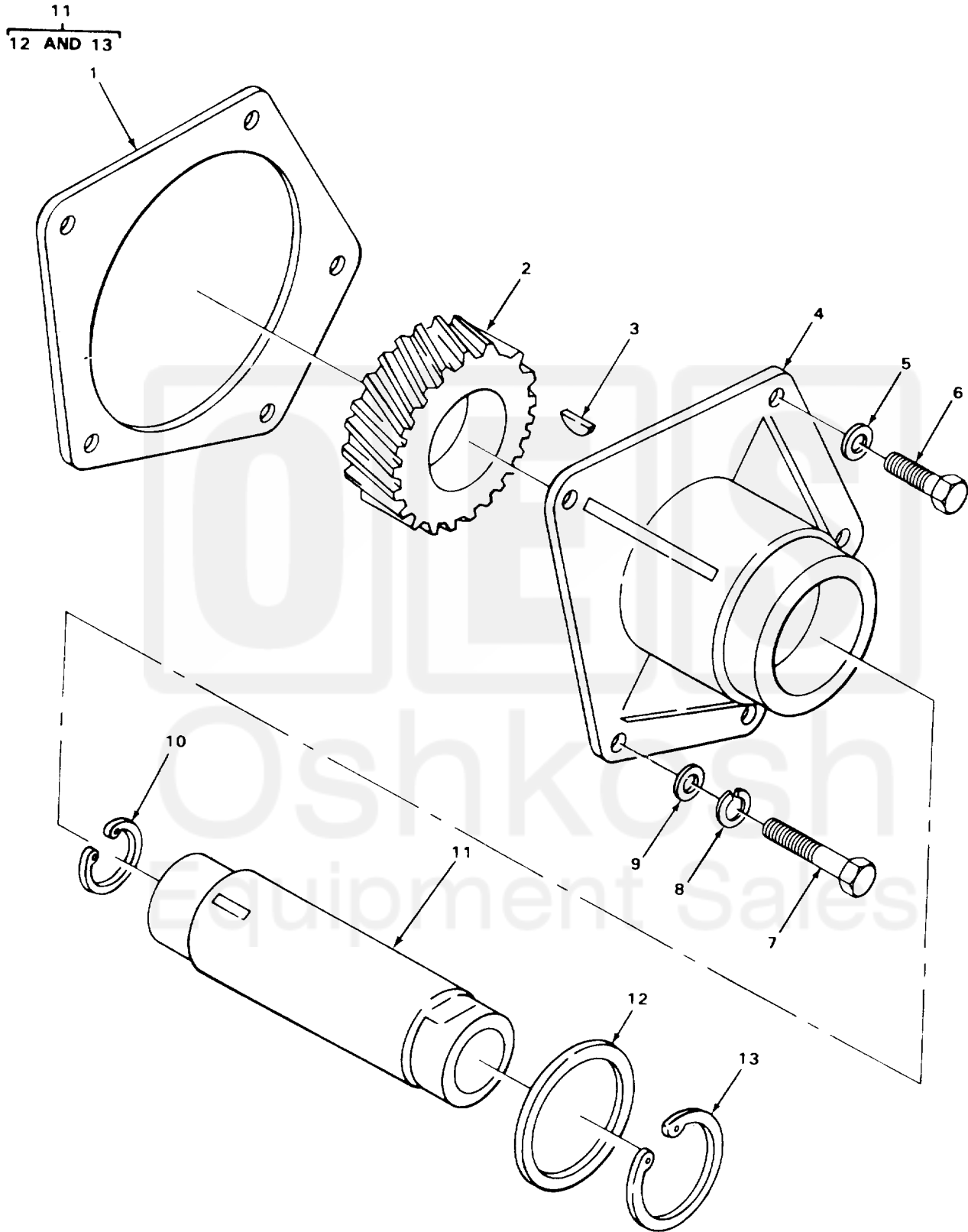
FIGURE 27. BLOWER DRIVE
